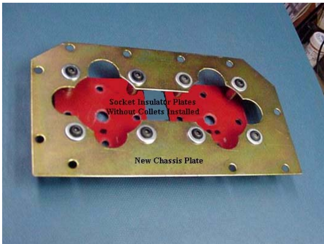
6I7BT Tube Socket Plate
